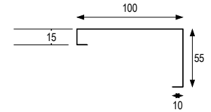
REINFORCING CHANNEL I DETAILS
